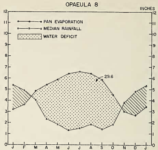
FIG. 13. Monthly water balance at Opaëula.
